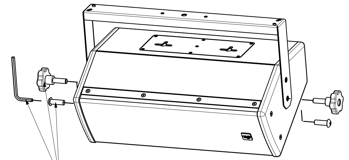
HORIZONTAL BRACKET ESD25 INCLUDING TWO SCREWS, TWO CONNECTION BOLTS AND ALLEN KEY
