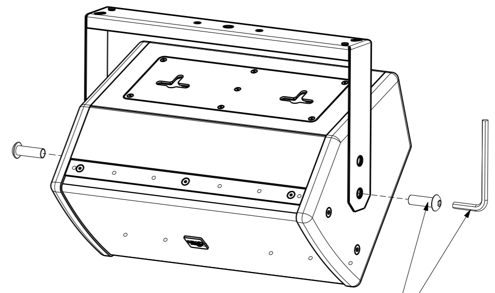
HORIZONTAL BRACKET ESD5 INCLUDING TWO SCREWS AND ALLEN KEY
