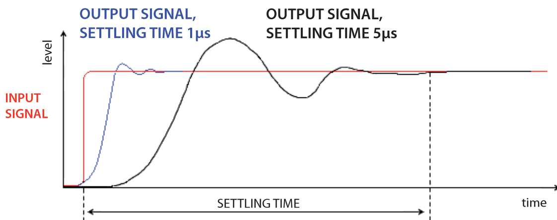
Settling time 5µs (black), 1µs (blue)
