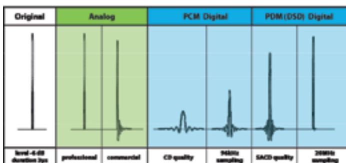
Figure B: Pulse response of an audio signal after transfer through various analog and digital systems.
